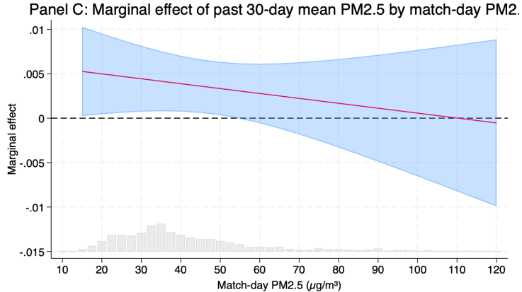
Figure 7. Marginal effect of past 30-day mean PM 2.5 on run-scoring probability, by match-day PM 2.5 level.
