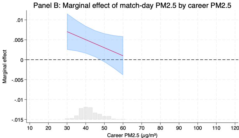
Figure 6. Marginal effect of match-day PM 2.5 by bowler's career mean (PM 2.5 j0 ). Median career exposure: 42 \mu\text{g m}^{-3} ; 95th percentile: 52 \mu\text{g m}^{-3} .
