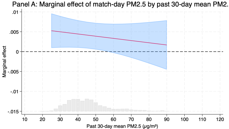
Figure 3. Marginal effect of match-day PM 2.5 on run-scoring probability by bowler's past 30-day mean PM 2.5 . Median past: 45 \mu\text{g m}^{-3} ; 95th percentile: 92 \mu\text{g m}^{-3} .
